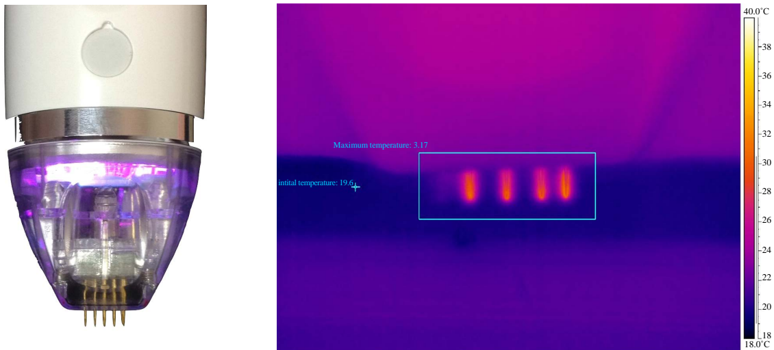
Figure 1. Left: EndyMed's Intensif Handpiece. Right: Thermal image of a treatment of laboratory skin model with impedance similar to dermal impedance (Flir Systems, ThermaCAM SC 640).
